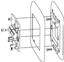
Vertical single gang box (wall plate and latches sold separately)
